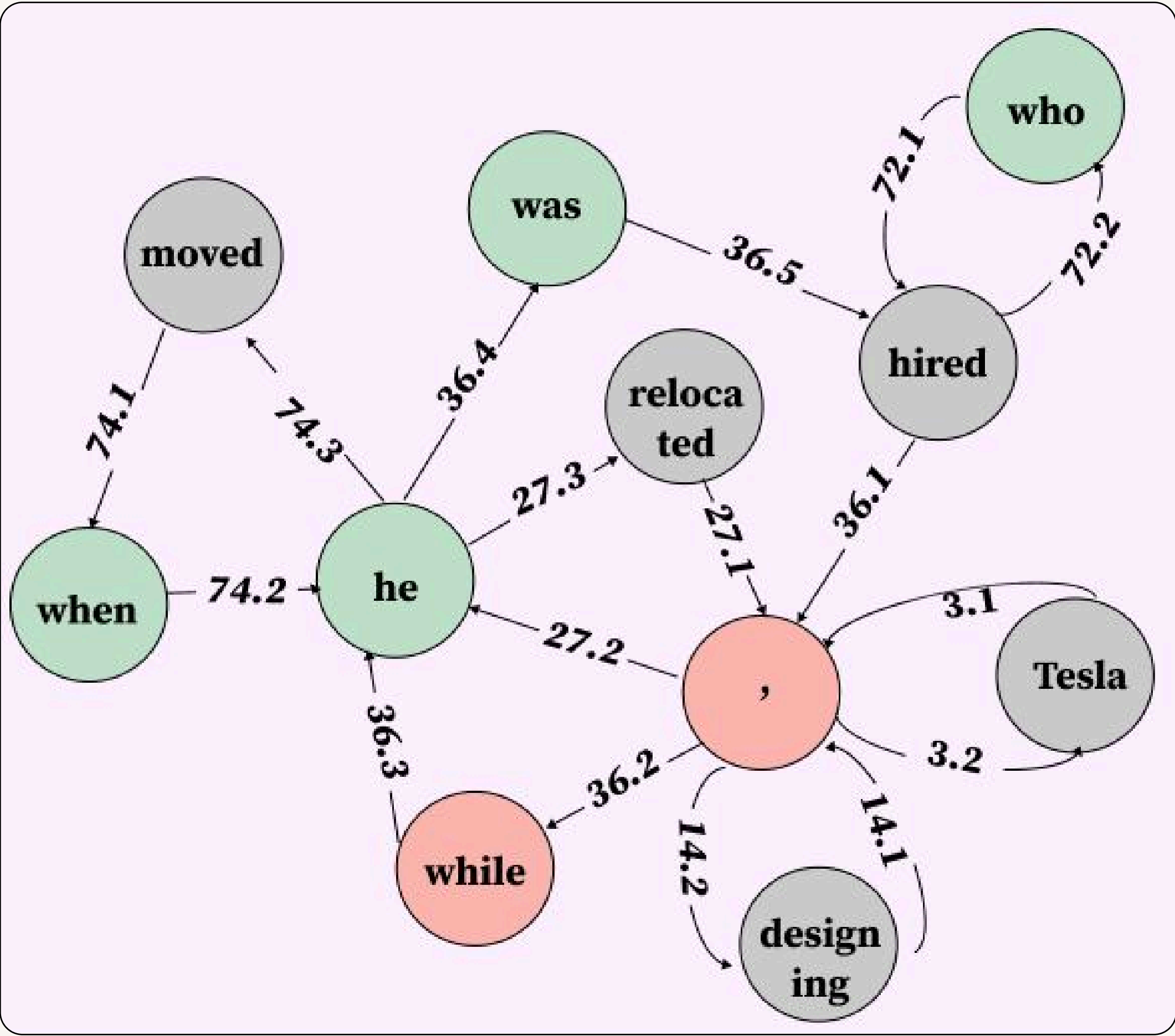
Formed interrogative directed weighted graph
